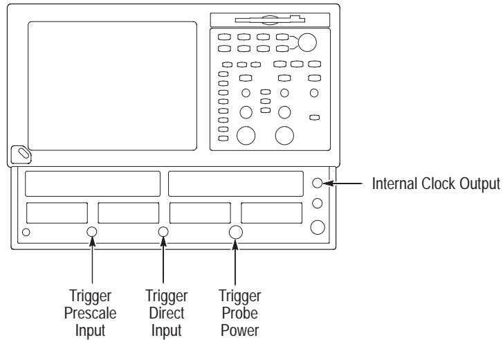
Figure 3-13: Trigger inputs
