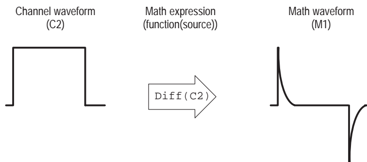
Figure 3–24: Functional transformation of an acquired waveform
